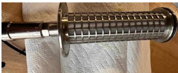
Figure 2. Filter Inspection
